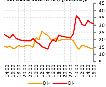
Directional Movement (7), посл. 4 д.
