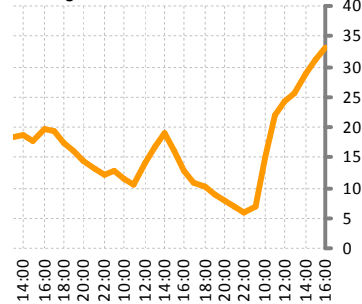
Average Directional Movement Index
