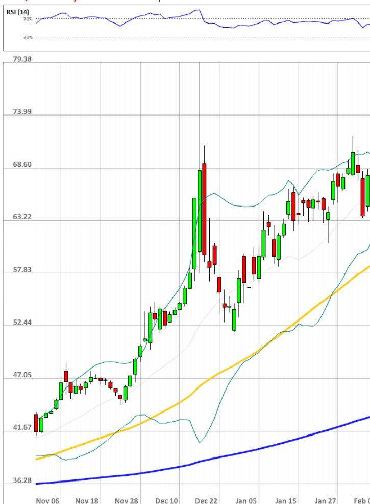
USD/RUB Daily Chart Current price: 66.14
